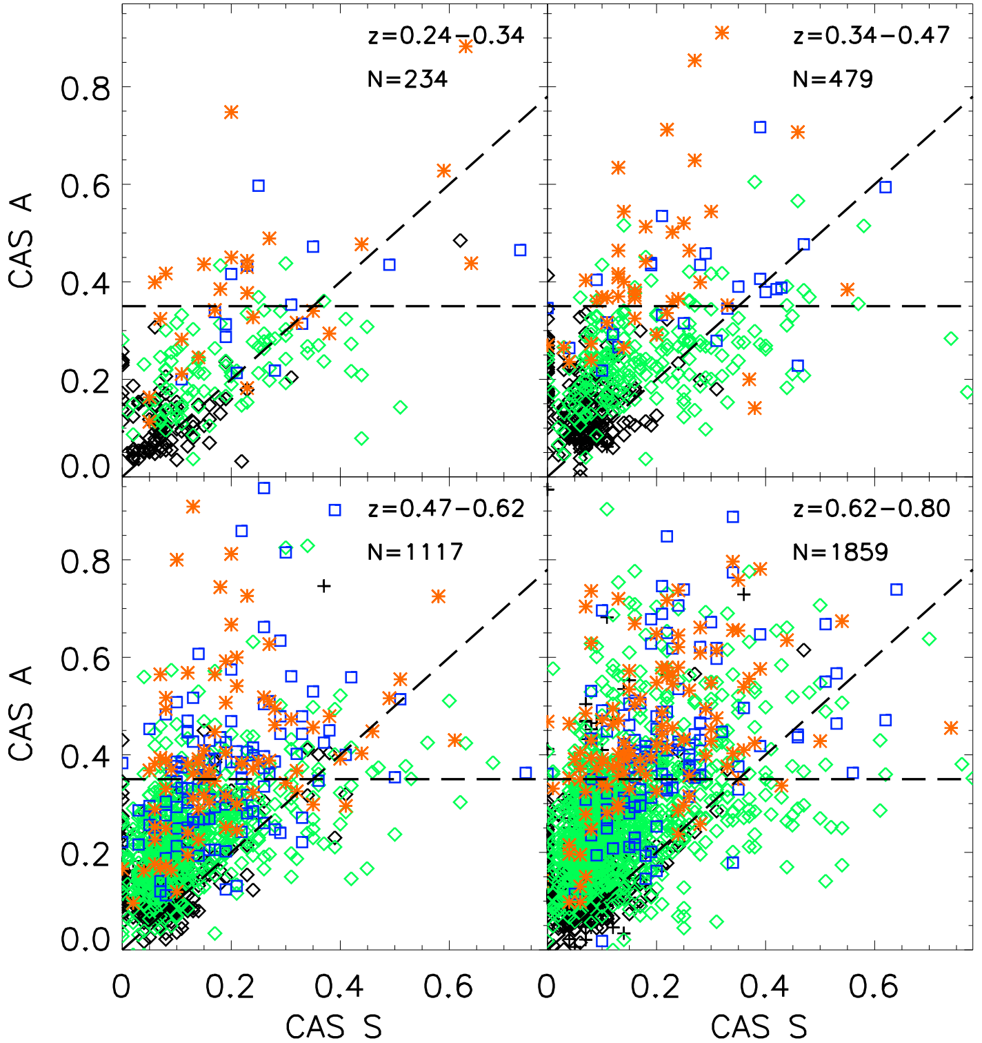
FIG. 7.— The CAS asymmetry A and clumpiness S parameters are plotted for intermediate mass ( M \geq 1 \times 10^9 M_\odot ) galaxies in the four redshift bins of Fig. 1, using the same color coding. Galaxies satisfying the CAS criterion ( A > 0.35 and A > S ) lie in the upper left hand corner, bracketed by the A = S diagonal line and the A = 0.35 horizontal line. The CAS criterion captures a fair fraction of the merging galaxies, but it also picks up “contaminants” in the form of non-interacting galaxies. This is further illustrated in Fig. 8.
