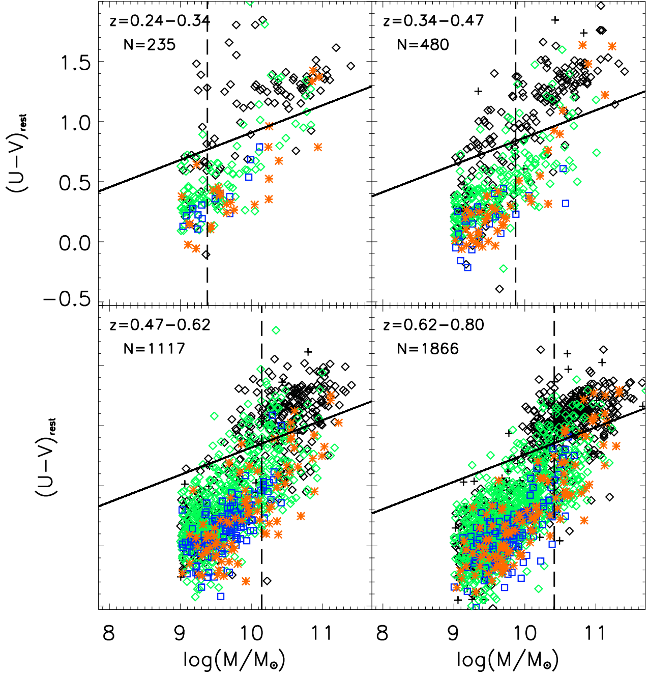
FIG. 1.— The rest-frame U - V color is plotted versus the stellar mass over z \sim 0.24\text{--}0.80 for the sample S2 of \sim 3698 galaxies with M \geq 1 \times 10^9 M_\odot . The four panels denote the four redshift bins, which span 1 Gyr each, and cumulatively cover the interval z \sim 0.24\text{--}0.80 ( T_{\text{back}} \sim 3\text{--}7 Gyr). N denotes the number of galaxies in each bin. The diagonal line marks the separation of the red sequence galaxies and the blue cloud galaxies at the average redshift z_{\text{ave}} of the bin. The vertical lines marks the mass completeness limit (Borch et al. 2006) for the red sequence galaxies, while the blue cloud galaxies are complete well below this mass. For the mass range M \geq 1 \times 10^9 M_\odot , the blue cloud is complete in our sample out to z \sim 0.80 , while the red sequence is incomplete in the higher redshift bins. Galaxies are coded according to their visual type (VT) in the F606W band: ‘Merging’ (orange stars), ‘Non-Interacting E+S0+Sa’ (black diamonds), ‘Non-Interacting Sb-Sc + Sd’ (green diamonds), and ‘Non-Interacting Irr1’ (blue squares).
