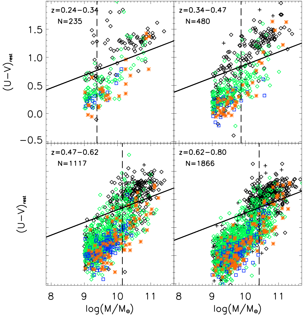
FIG. 1.— The rest-frame U - V color is plotted versus the stellar mass over z \sim 0.24-0.80 for the sample S2 of \sim 3698 galaxies with M \geq 1 \times 10^9 M_\odot . The four panels denote the four redshift bins, which span 1 Gyr each, and cumulatively cover the interval z \sim 0.24-0.80 ( T_{\text{back}} \sim 3-7 Gyr). N denotes the number of galaxies in each bin. The diagonal line marks the separation of the red sequence galaxies and the blue cloud galaxies at the average redshift z_{\text{ave}} of the bin. The vertical lines marks the mass completeness limit (Borch et al. 2006) for the red sequence galaxies, while the blue cloud galaxies are complete well below this mass. For the mass range M \geq 1 \times 10^9 M_\odot , the blue cloud is complete in our sample out to z \sim 0.80 , while the red sequence is incomplete in the higher redshift bins. Galaxies are coded according to their visual type (VT) in the F606W band: ‘Mergers’ (orange stars), ‘Non-Interacting E+S0+Sa’ (black diamonds), ‘Non-Interacting Sb-Sc + Sd’ (green diamonds), and ‘Non-Interacting Irr1’ (blue squares).
