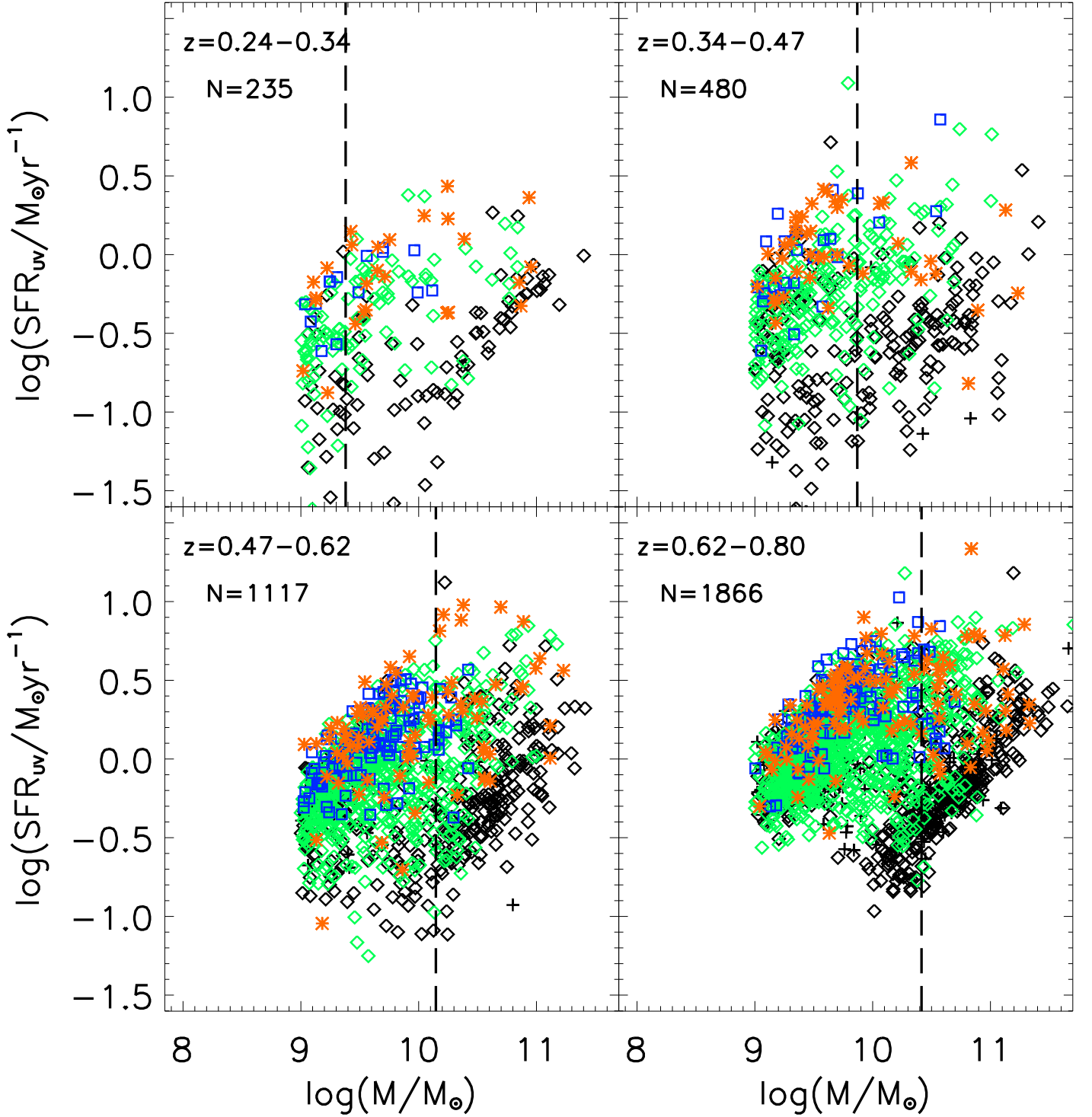
FIG. 13.— The UV-based star formation rate is plotted versus the stellar mass over z \sim 0.24\text{--}0.80 for the sample S2 of galaxies with M \geq 1 \times 10^9 M_\odot . The four panels show the four redshift bins, which span 1 Gyr each, and cumulatively cover the interval z \sim 0.24\text{--}0.80 ( T_{\text{back}} \sim 3\text{--}7 Gyr). N denotes the number of galaxies plotted in each bin. Galaxies are coded as in Fig. 1, with merging systems denoted by orange stars. The average SFR and total SFR density in both the UV and the IR, are further illustrated in Fig. 14 and Fig. 16.
