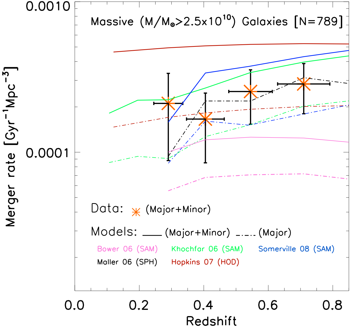
FIG. 12.— As in Figure 11, but now comparing the empirical rate R (orange stars) of mergers with mass ratio M1/M2 > 1/10 among high mass galaxies to the rate of (major+minor) mergers (solid lines; stellar mass ratio M1/M2 > 1/10 ) predicted by different \Lambda CDM-based simulations of galaxy evolution.
