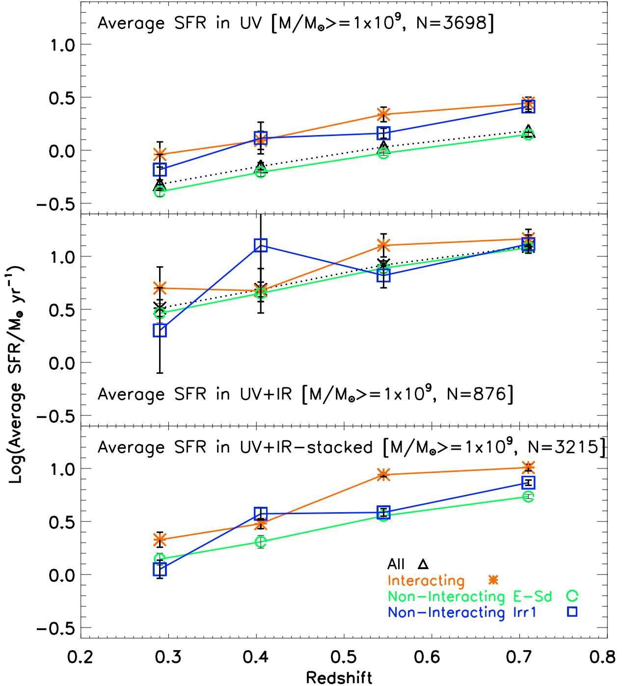
Fig. 13.— The average SFR of interacting, ‘non-interacting E-Sd’, and ‘non-interacting Irr1’ galaxies are compared over z \sim 0.24 – 0.80 for intermediate mass ( M \geq 1.0 \times 10^9 M_{\odot} ) galaxies. N denotes the number of galaxies used. The average UV-based SFR (top panel; based on 3698 galaxies), average UV+IR-based SFR (middle panel; based on only the 876 galaxies with 24 \mu m detections), and average UV+IR-stacked SFR (based on 3215 galaxies with 24 \mu m coverage) are shown. In all these cases, the average SFR of interacting galaxies is only modestly enhanced compared to non-interacting galaxies over z \sim 0.24 – 0.80 (lookback time \sim 3 – 7 Gyr).
