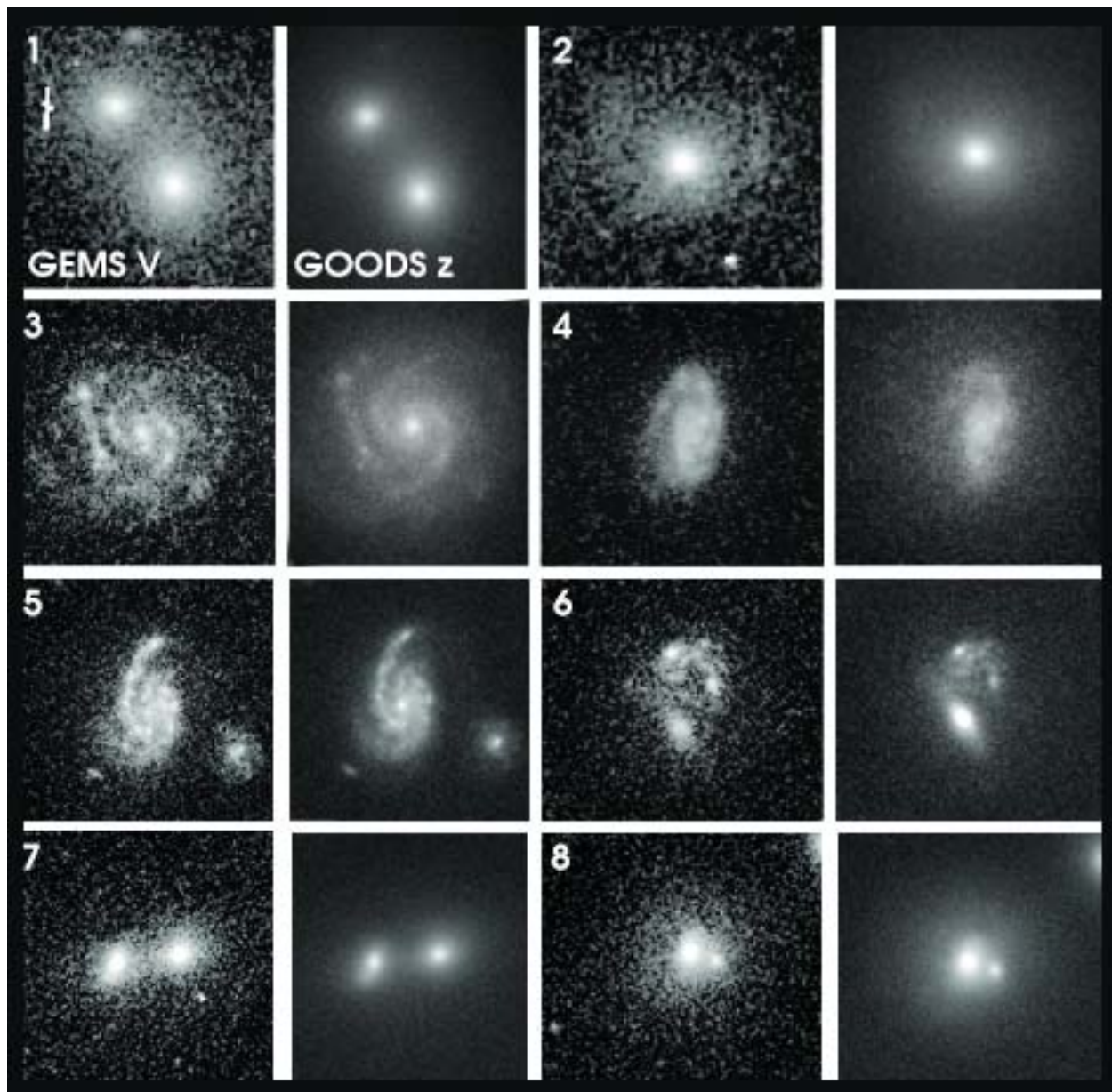
Fig. 5.— This montage illustrates a test for bandpass shift and surface brightness dimming. It compares the bluer shallower GEMS F606W images ( V band; pivot \lambda \sim 5915 \text{ \AA} ) and deeper redder GOODS F850LP ( z band; pivot \lambda \sim 9103 \text{ \AA} ) images of typical interacting and non-interacting galaxies in the last redshift bin ( z \sim 0.60 to 0.80 ), where bandpass shift and surface brightness dimming are expected to be most severe. In this redshift bin, the rest-frame wavelength traced by the GEMS images shift from optical to violet/near-UV ( 3700 \text{ \AA} to 3290 \text{ \AA} ). However, while the GOODS images have higher S/N, and trace redder older stars, they do not reveal dramatically different morphologies from those in the GEMS F606W images. A statistical analysis is shown in Table 3.
