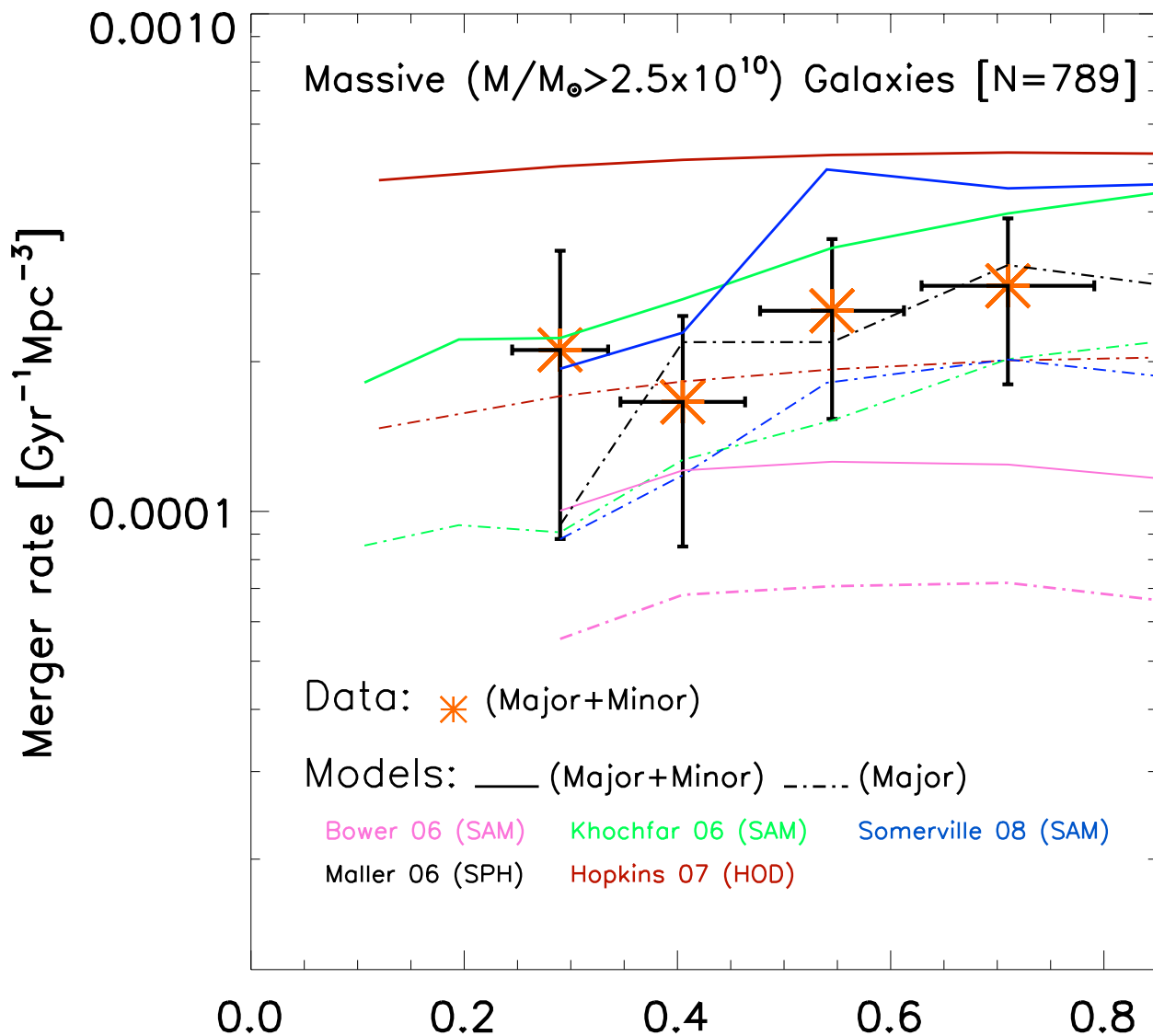
Fig. 11.— The empirical rate R (orange stars) of mergers with mass ratio M1/M2 > 1/10 among high mass galaxies is compared to the rate of (major+minor) mergers (solid lines; stellar mass ratio M1/M2 > 1/10 ) predicted by different \Lambda CDM-based simulations of galaxy evolution, including the halo occupation distribution (HOD) models of Hopkins et al. (2007); semi-analytic models (SAMs) of Somerville et al. (2008), Bower et al. (2006), and Khochfar & Silk (2006); and smoothed particle hydrodynamics (SPH) cosmological simulations from Maller et al. (2006) (see § 4.5).
