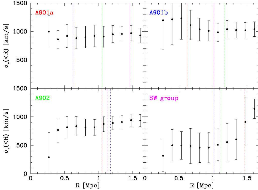
Fig. 10.— Integrated velocity dispersion profiles for A901a, b and A902 clusters, and associated SWG from kinematic modeling using 2dF redshifts (Gray et al. 2008b?). The integrated velocity dispersion profiles are relatively flat. Calculations of the local velocity dispersion profile [TO BE UPDATED WITH LOCAL VDP FROM MEGHAN]in the cluster core, outer region, and cluster outskirts are needed in order to make the final determination if the velocity dispersion of galaxies falls between the cluster core and outskirts. If this is true, the galaxy velocity dispersion may be low enough to enable galaxies to become gravitationally bound and interact.
