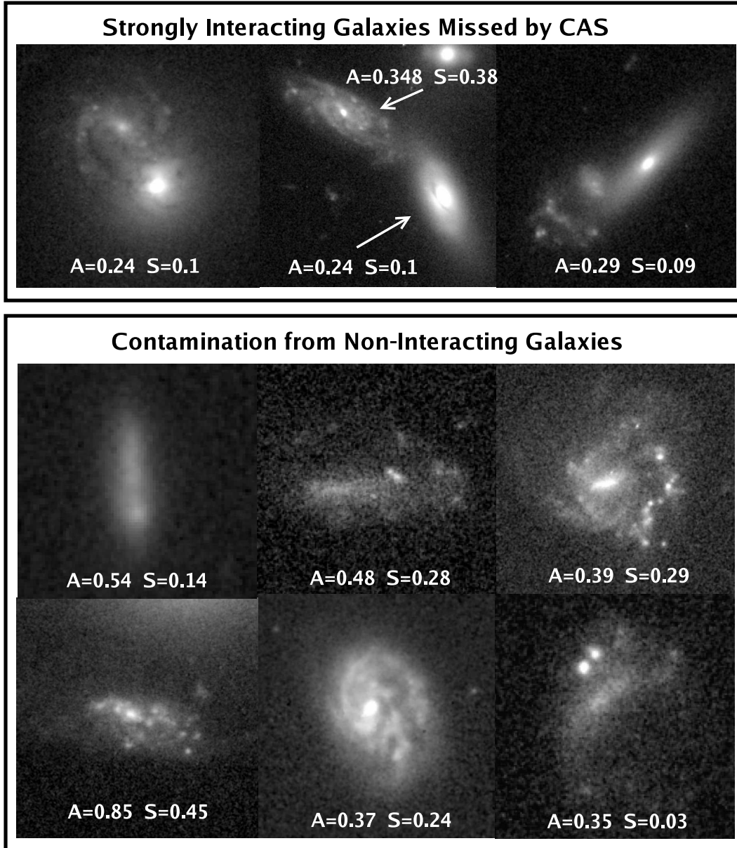
Fig. 6.— The top panel shows examples of strongly interacting missed by CAS criterion ( A > S and A > 0.35 ). Features of these systems include double nuclei, tidal bridges, and tidal debris. The lower panel show some ‘Non-Interacting’ contaminants CAS picked up due to small-scale asymmetries from SF, large dust lanes, and the absence of a clear center, all leading to a larger A value.
