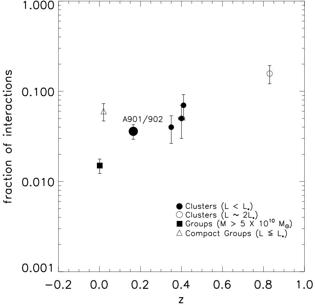
Fig. 12.— Comparisons of our observed fraction of strongly interacting galaxies with other studies of clusters, groups, and field galaxies. Filled circles are for cluster data points of intermediate luminosity ( L < L_* and/or M = 1 \times 10^9 to a few \times 10^{10} M_\odot ), and the cluster data points are in order of increasing redshift: this study of A901/902 (for M_V \sim -18.5 to -24 and M_* = 1 \times 10^9 to a few \times 10^{10} M_\odot ); Couch et al. (1998; L < 2L_* ), Oemler et al. (1997; lower limit of f for M_V < -19 ), Dressler et al. (1994; M_V < -18.5 ). The Tran et al. (2005b) point at z = 0.83 (open circle) is for a cluster sample of luminous ( M_B \sim -22 and L \sim 2L_* ) galaxies. The group point (filled square) is from McIntosh et al. (2007) for galaxy masses above 5 \times 10^{10} M_\odot . The Hickson compact group point (open triangle) is from Zepf et al. (1993) and is for galaxies of luminosities L \leq L_* .
