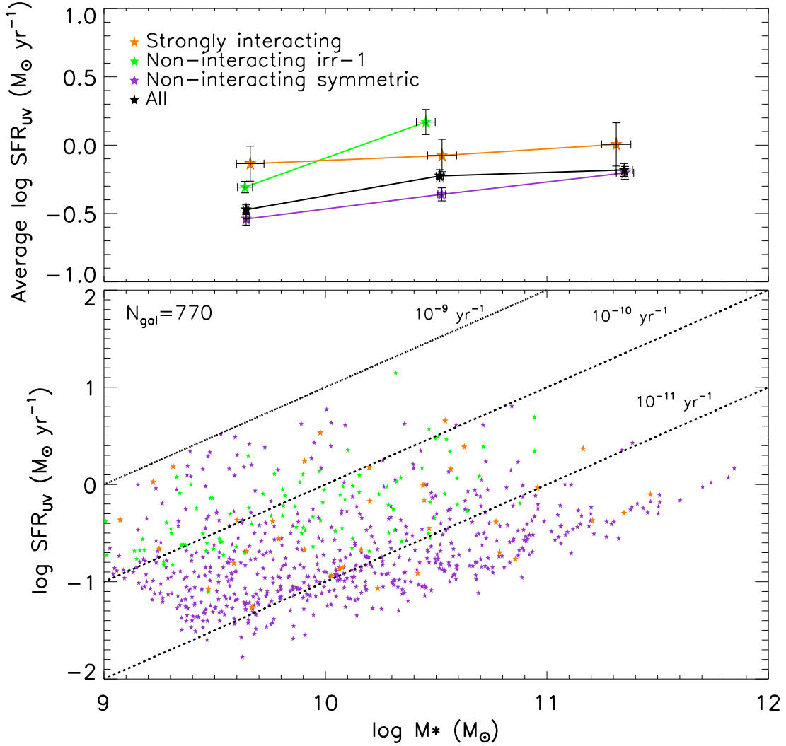
Fig. 14.— Top panel: The average UV-based SFR is plotted versus stellar mass for all galaxies and for galaxies of different visual classes. For the few strongly interacting galaxies present, the average SFR UV is enhanced by a modest factor of \sim 2 -3 compared to the Non-interacting Symmetric galaxies and most of the Non-interacting Irr-1 galaxies. Lower panel: The UV-based SFR is plotted versus stellar mass. Galaxies are coded according to their visual classes: Strongly interacting, Non-interacting Irr-1, and Non-interacting Symmetric. Loci of constant specific SFR are marked in units of yr -1 .
