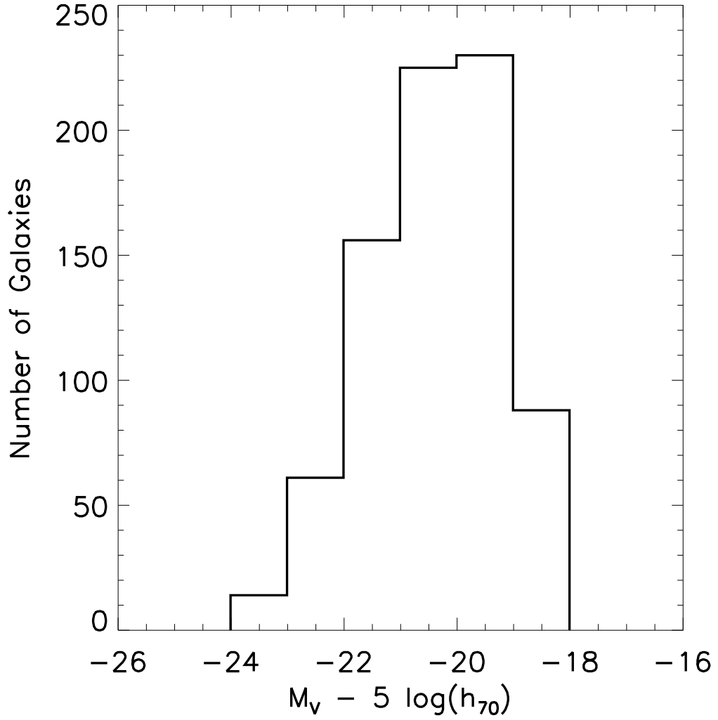
Fig. 1.— Absolute magnitude distribution of the A901/902 supercluster sample of bright ( M_V < -18 ), intermediate mass ( M > 1 \times 10^9 M_\odot ) galaxies (N=774 galaxies).
