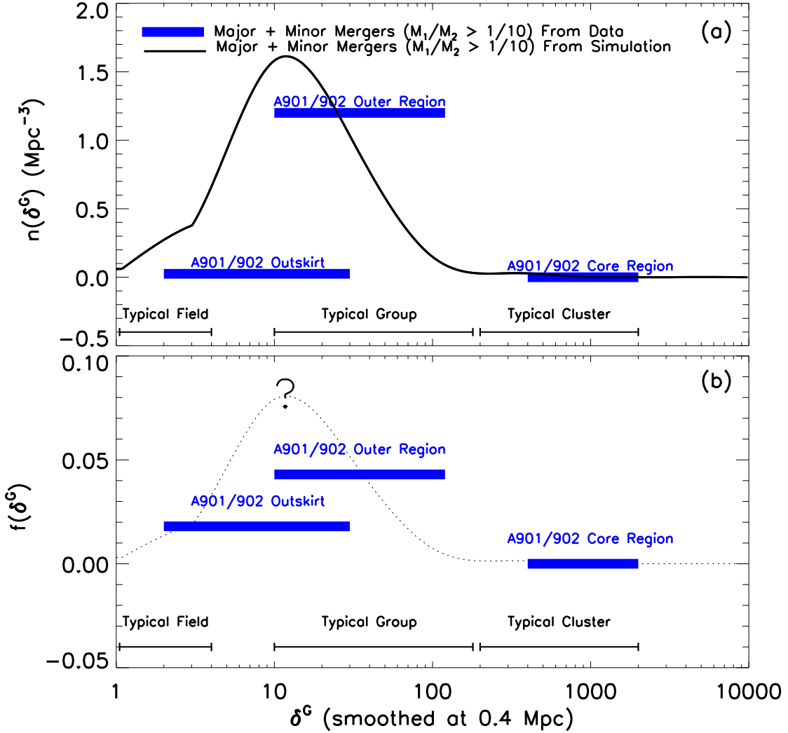
Fig. 11.— Model predictions are shown from N -body simulations of the STAGES A901/902 supercluster (van Kampen et al. 2008, in prep.). A stellar mass cut of ( M > 1 \times 10^9 M_\odot ) is applied. This figure shows model predictions for the number density ( n(\delta^G) ; (a) ) and fraction ( f(\delta^G) ; (b) ) [TO BE UPDATED WITH NUMBERS FROM EELCO]) of galaxy mergers of mass ratio M_1/M_2 > 1/10 , as a function of environment, as characterized by the local overdensity ( \delta^G ). The latter is calculated by smoothing the density of dark matter halos with a Gaussian of width 0.4 Mpc to take out the effect of individual galaxies. Typical values of \delta^G are \sim 10 - 100 for group overdensities, \sim 200 at the cluster virial radius, and > 1000 in core of rich clusters. The highest number of mergers is found in groups, but as a groups fall into a higher density cluster environment, the merger rate goes down. In cluster cores, mergers are rare. The solid blue regions show the range for number density ( n_{\text{merg}} ) and fraction of mergers (Table 7) we observe in the cluster core, virial radius, and outskirts in A901/902 (§ 4.4).
