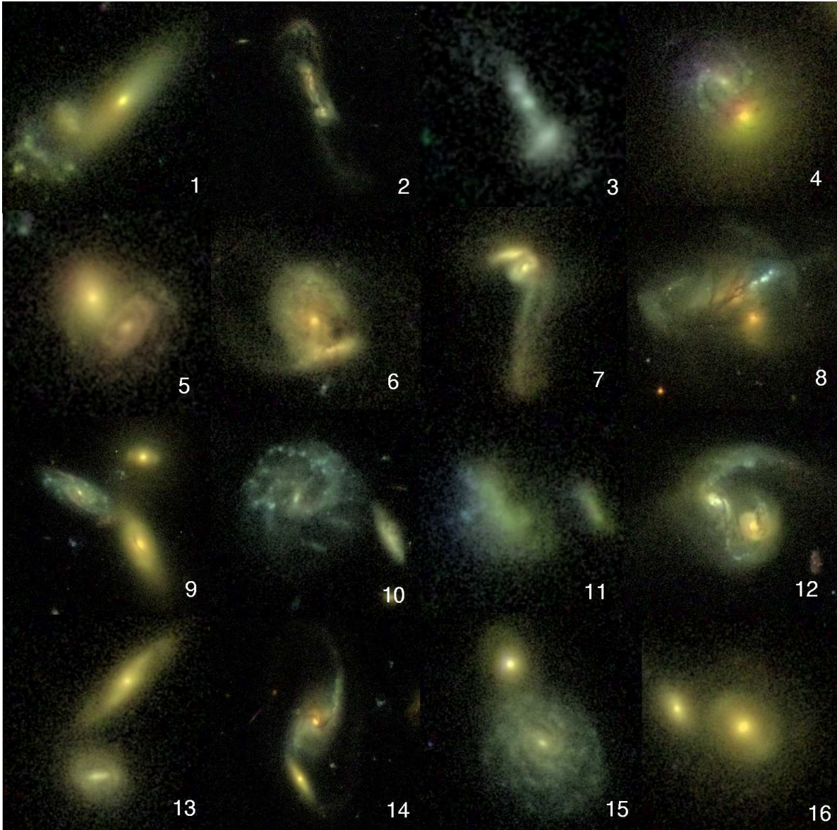
Fig. 3.— Examples of galaxies visually classified as strongly interacting (‘Int’), divided into ‘Type 1’ and ‘Type 2’ (§ 3.2). ‘Int Type 1’ systems (cases 1-8) host strong externally-triggered morphological distortions, such as tidal tails, arcs, shells, ripples, warps, tidal debris in body of galaxy, offset rings, extremely asymmetric star formation, spiral arms on only one side of the disk, and double nuclei. In contrast, ‘Int Type 2’ galaxies do not have strong morphological distortions (cases 9-16), but they are considered to be strongly interacting because they have a companion which satisfies 3 criteria: it has project separation d \lesssim 10 kpc, the same COMBO-17 spectrophotometric redshift, and gives a stellar mass ratio M_1/M_2 > 1/10 . Among these interacting systems, note potential major (9, 12, 13, 14, 15) and minor (10, 11, 16) interactions, as well as more ambiguous cases (1-8) that could be either major or minor (§ 4.1).
