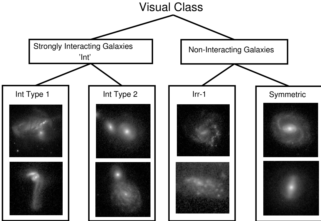
Fig. 2.— In our visual classification scheme (§ 3.2), galaxies are classified as strongly interacting (‘Int’), non-interacting, or unclassifiable. The strongly interacting galaxies (‘Int’) consists of ‘Type 1’ and ‘Type 2’ systems (see Fig. 3). ‘Int Type 1’ systems host strong externally-triggered morphological distortions, such as tidal tails, shells, ripples, warps, strongly asymmetric tidal debris and distortions in the disk, and double nuclei inside a common envelope. In contrast, ‘Int Type 2’ galaxies do not have strong morphological distortions, but they are considered to be strongly interacting because they have a companion which satisfies 3 criteria: it has project separation d \lesssim 10 kpc, the same COMBO-17 spectrophotometric redshift, and gives a stellar mass ratio M_1/M_2 > 1/10 . The non-interacting galaxies consists of ‘Irr-1’ and ‘Symmetric’ systems. Irr-1 exhibit internally-triggered asymmetries, due to SF typically on scales of a few hundred parsecs. ‘Symmetric’ systems are relatively undistorted and are not associated with any overlapping companion.
