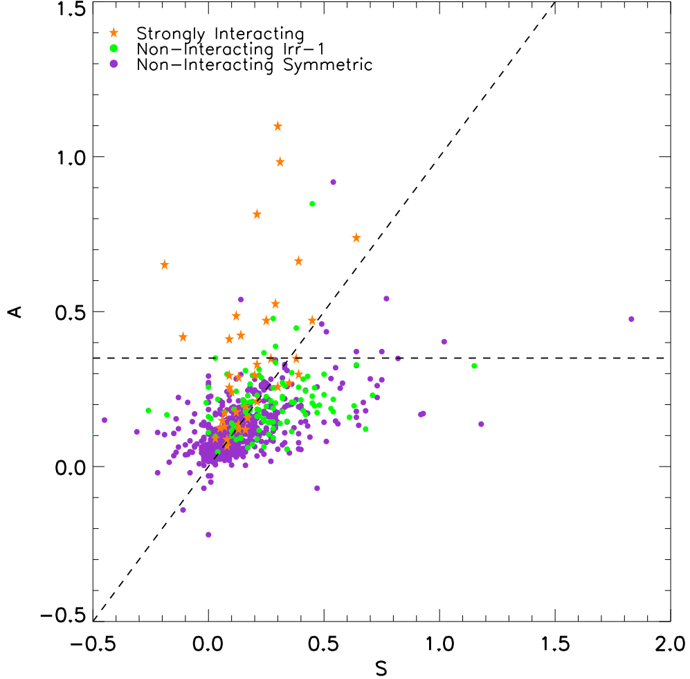
Fig. 5.— Bright, intermediate mass ( M_V < -18 ; M \geq 1 \times 10^9 M_\odot ) galaxies of different visual classes (Strongly interacting, Non-interacting Irr-1, & Non-interacting Symmetric) are shown in the CAS A versus S plane. The 21 galaxies satisfying the CAS merger criterion ( A > S and A > 0.35 ) lie on the upper left corner of the diagram. The CAS merger criterion recovers 13/38 ( 34^{+5\%}_{-3\%} ) of the galaxies visually classified as strongly interacting. Furthermore, there is a significant level of contamination: 8/21 ( 38^{+16\%}_{-5\%} ) of the systems picked up by the CAS criterion are visually classified as non-interacting irr-1 and Non-interacting Symmetric.
