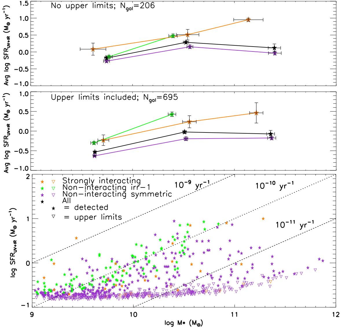
Fig. 15.— Top panel: The average UV+IR-based SFR is plotted versus stellar mass for all galaxies and for galaxies of different visual classes, upper limits not included. Middle panel: The average UV+IR-based SFR is plotted versus stellar mass for all galaxies and for galaxies of different visual classes, upper limits included. For the few strongly interacting galaxies present, the average \text{SFR}_{\text{UV+IR}} is enhanced by a \sim 3 to 4 compared to the Non-interacting Symmetric galaxies and most of the Non-interacting Irr-1 galaxies regardless of . Bottom panel: The UV+IR-based SFR is plotted versus stellar mass. Galaxies are coded according to their visual classes: Strongly interacting, Non-interacting Irr-1, and Non-interacting Symmetric. Loci of constant specific SFR are marked in units of \text{yr}^{-1} . The inverted triangles denote upper limits for galaxies where there was no 24 micron detection and where we used the detection limit.
