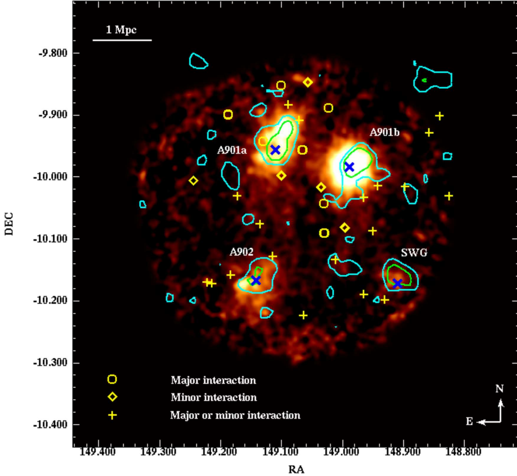
Fig. 8.— The distribution of strongly interacting galaxies (coded as yellow diamonds, ‘+’, and circles) is overlaid on the ICM gas density (yellow-orange scale). Following Heymans et al. (2008), we show DM masses in terms of the signal-to-noise of the weak lensing detection. The cyan and green contours enclose roughly 6h^{-1}10^{13}M_{\odot} and 3.5h^{-1}10^{13}M_{\odot} for A901a and A901b, and roughly 3h^{-1}10^{13}M_{\odot} and 1.5h^{-1}10^{13}M_{\odot} for the lower mass A902 and South West Group (SWG). The different symbols represent our best attempt to separate the strongly interacting galaxies into ‘major’ (circles), ‘minor’ (diamonds), and ‘major or minor’ (+) interactions (§ 4.3). Strongly interacting galaxies are located in the outer region of the cluster ( 0.25 \text{ Mpc} < R \leq 1.2 \text{ Mpc} ).
