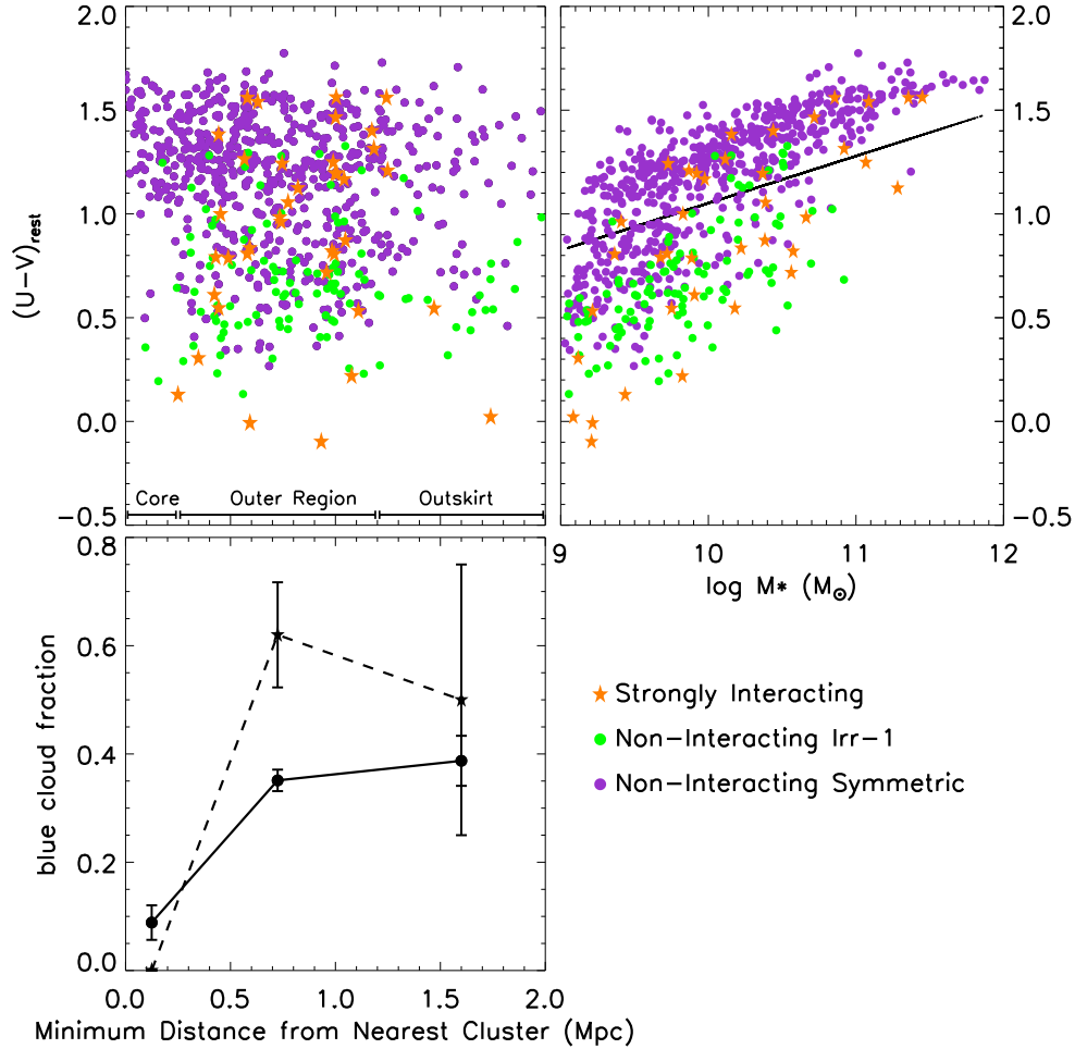
Fig. 13.— Top Left: The rest-frame U - V color of galaxies is plotted against their minimum distance from the nearest cluster center. Top Right: The rest-frame U - V color is plotted against stellar masses for galaxies of different visual classes (Strongly interacting, Non-interacting Irr-1, and Non-interacting Symmetric). The black solid lines separate the blue cloud and red sequence. For M \geq 1 \times 10^9 M_\odot systems, we find that 61 \pm 14\% (23/38) of the strongly interacting galaxies lie on the blue cloud, compared to 34 \pm 7\% (257/732) for non-interacting galaxies. There is an excess of blue galaxies among interacting systems. Bottom Left: The fraction of all galaxies on the blue cloud (solid line), and the fraction of strongly interacting galaxies on the blue cloud (dotted line) both rise as a function of clustocentric radius (Table 7). The increase is more pronounced for the fraction of blue interacting galaxies, which rises from 0 to 0.62 \pm 0.15 to 0.50 \pm 0.25\% (Table 7) in the cluster core ( R \leq 0.25 Mpc) to the outer region ( 0.25 Mpc < R \leq 1.2 Mpc) to the outskirts region ( 1.2 Mpc < R \leq 2 Mpc).
