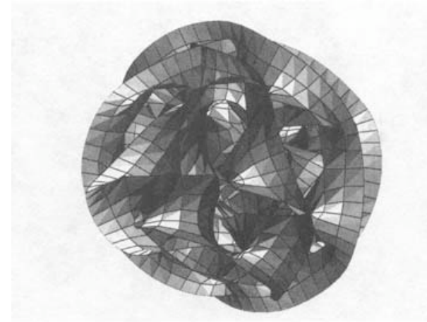
Representation of a Calabi-Yau space, with 6 wrapped-up extra dimensions. From Brian Green: The Elegant Universe.
