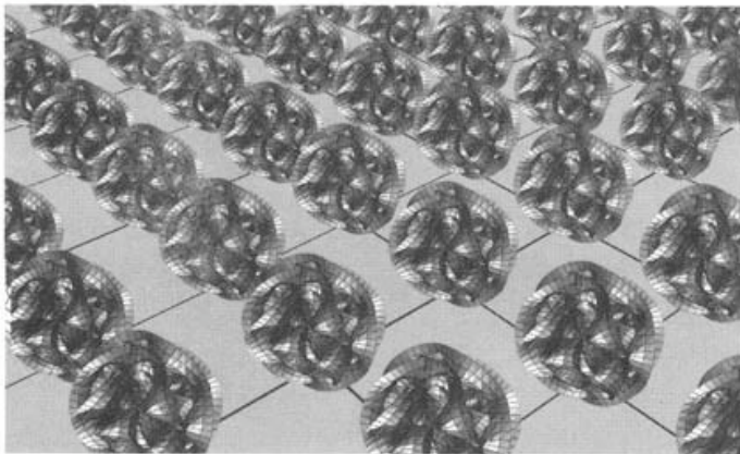
At each point in the 2D space (not just at the intersections of grid lines), there is a little 6D Calabi-Yau space of six wrapped-up extra dimensions. From Brian Green: The Elegant Universe.
