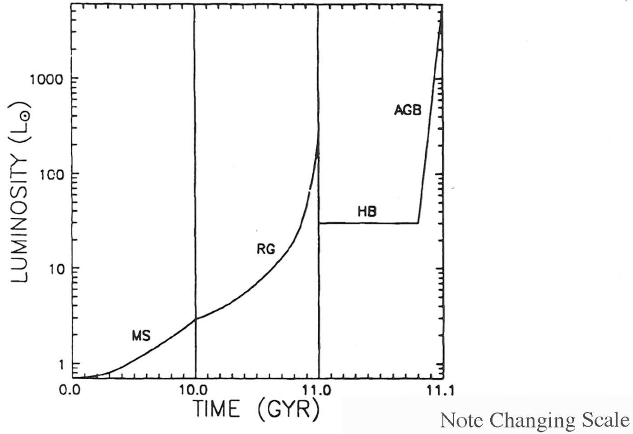
FIG. 1. Luminosity evolution of a 1 M_{\odot} star of solar composition. Note that the scale is broken at 10 and 11 Gyr. The discontinuity at 11 Gyr is real and is due to the helium flash. The phases are: MS = main sequence, RG = red giant, HB = horizontal branch, and AGB = asymptotic giant branch. The final white dwarf phase is not illustrated. Details of the evolution during the HB and AGB phases are omitted.
