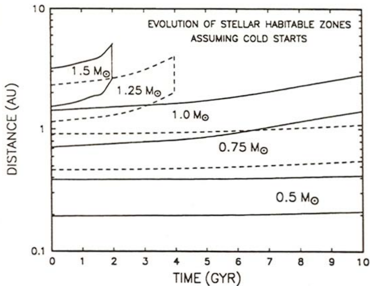
FIG. 5. Evolution of the H around stars of different masses assuming that co starts are possible. Case critical fluxes were used and the evolution was truncated at the end of the main sequence phase.
