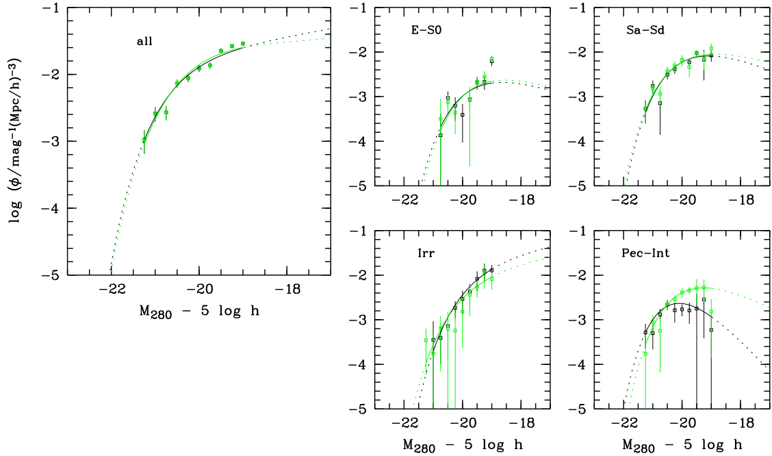
FIG. 8.— Near-UV luminosity functions from GOODS-shallow vs. GOODS-deep: The image depth influences our morphological classifications, an effect which propagates into the luminosity functions by type. Here, we compare the LFs derived from the 290 galaxies from the GOODS area using both GEMS-depth and GOODS-depth data to separate classification differences from cosmic variance. The GEMS result is shown in black and the GOODS result in grey. The major difference is that the LF of Pec-Int galaxies is increased at the faint end, while irregulars are lower by a similar amount.
