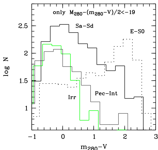
FIG. 6.— The rest-frame color distribution for different morphological types: Spheroids (E-S0) are predominantly red, irregulars almost uniquely very blue. Spirals and major mergers (Pec-Int) have somewhat similar distributions, with mostly blue objects and a tail to the red. Here, we only used galaxies from a brighter subsample that is at least 90% complete.
