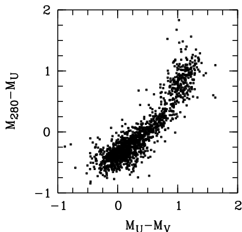
FIG. 4.— Rest-frame colors: The sample galaxies form almost a one-parameter family in near-UV-optical rest-frame colors. The bimodality can be seen as well.
