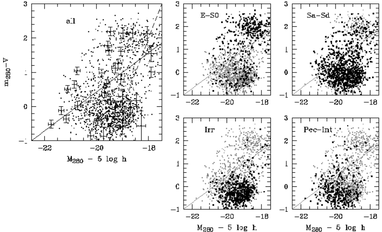
FIG. 5.— Color-magnitude diagram: Left : The parent sample with 1483 galaxies. Error bars are given for a randomly-chosen subsample; the error bars include expected systematic biases. The solid line roughly represents galaxies with constant mass of 10^{10} h^{-2} M_{\odot} , following Bell & de Jong (2001). The dashed line delineates a subsample with > 90\% completeness. Right : Four panels showing the distribution of colors and magnitudes of the four different morphological types from all three classifiers combined (black dots) on top of the parent sample (grey background dots).
