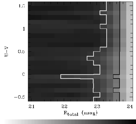
FIG. 3.— Sample completeness: Monte-Carlo simulations of the COMBO-17 survey with classification and redshift estimation yield this map of completeness for galaxies at 0.65 < z < 0.75 . Dark grey denotes high completeness, light grey resembles low completeness. Lines are drawn at 50% completeness (black) and 90% (white). At R < 23 the sample is more than 90% complete, at R = 23.7 still \sim 50\% of the galaxies are included. At R > 24 no galaxy is included, because of the R_{\text{aper}} < 24 selection cut.
