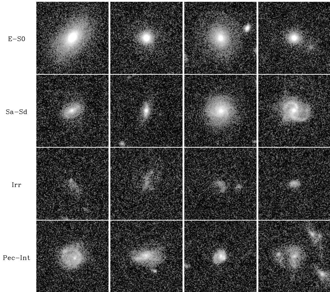
FIG. 1.— HST/ACS F850LP example images of the four broad type bins types; each class has four examples. Panels measure 6'' \times 6'' , corresponding to roughly 45 \text{ kpc} \times 45 \text{ kpc} . From top row to bottom row: E-S0 — Sa-Sd — Irr — Pec/Int.
