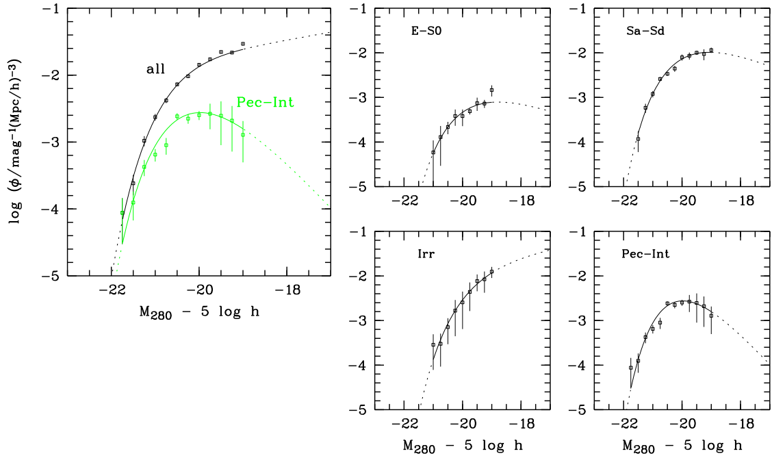
FIG. 7.— Near-UV luminosity functions from GEMS: Left : Parent sample with all galaxies, compared to clearly-interacting galaxies. Lines are best-fitting Schechter functions. Right : The four morphological types, E-S0 = spheroids, Sa-Sd = spiral galaxies, Irr = irregulars, Pec-Int = clearly interacting galaxies. Error bars are from Poisson noise or author-to-author variation from their independent morphological classifications, whichever is greater.
