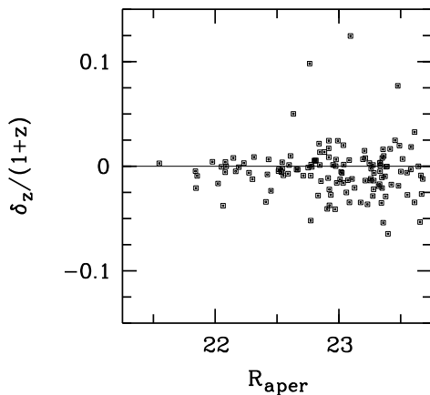
FIG. 2.— Redshift errors: The VVDS survey provides redshifts with > 95\% reliability for 152 of the 1483 galaxies in our sample. Three outliers can be seen with redshift errors on the order of \delta_z \sim 0.1 . The bulk of the sample (98%) have a mean offset from the spectroscopic redshift of \langle \delta_z / (1+z) \rangle = -0.006 and an RMS scatter of 0.020 in terms of \delta_z / (1+z) .
