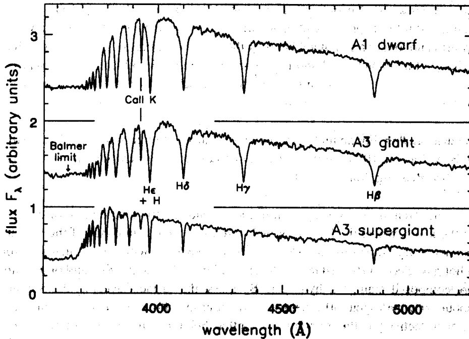
Figure 1.2 Spectra of an A1 dwarf, an A3 giant, and an A3 supergiant: the most luminous star has the narrowest spectral lines – G. Jacoby et al. , spectral library.
