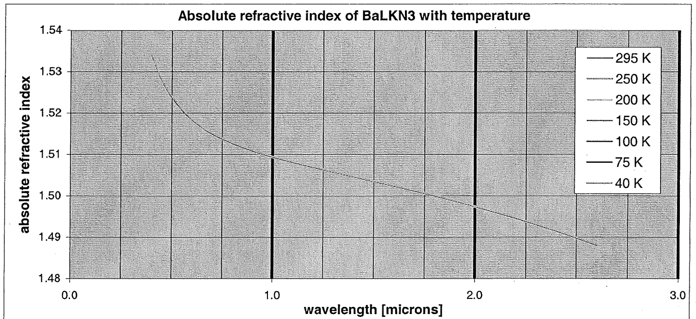
Figure 4: Measured absolute refractive index of BaLKN3 as a function of wavelength for selected temperatures
