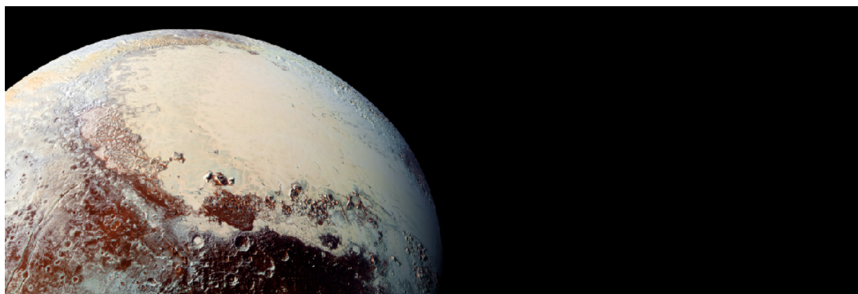
Figure 7.6. Pluto Close-up. This intriguing image from the New Horizons spacecraft, taken when it flew by the dwarf planet in July 2015, shows some of its complex surface features. The rounded white area is temporarily being called the Sputnik Plain, after humanity's first spacecraft. (credit: modification of work by NASA/Johns Hopkins University Applied Physics Laboratory/Southwest Research Institute)
