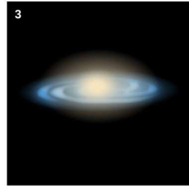
3 Large bulge of ancient stars dominates galaxy.
