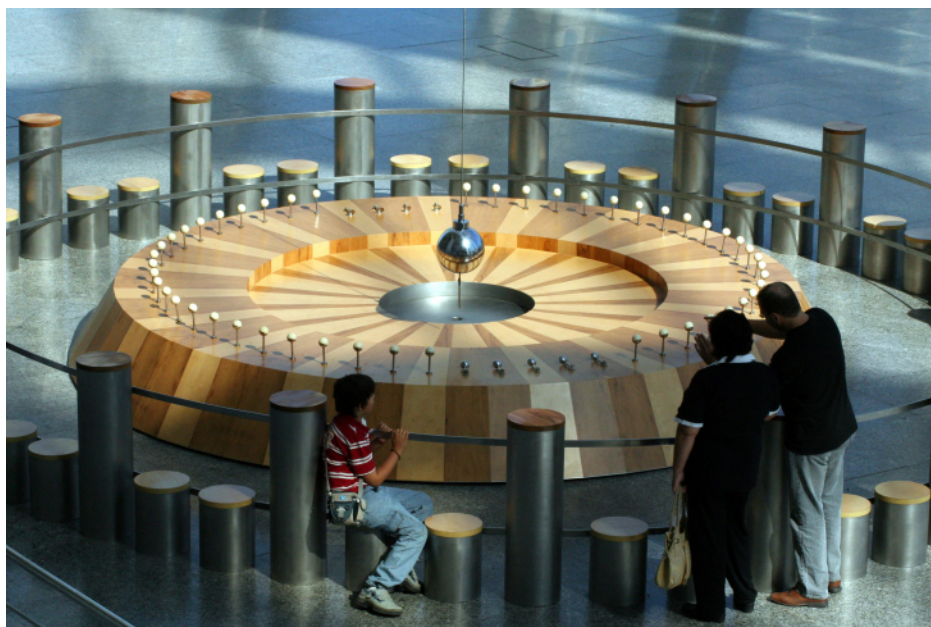
Figure 4.4. Foucault's Pendulum. As Earth turns, the plane of oscillation of the Foucault pendulum shifts gradually so that over the course of 12 hours, all the targets in the circle at the edge of the wooden platform are knocked over in sequence. (credit: Manuel M. Vicente)
