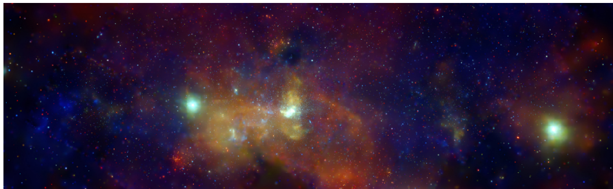
Figure 25.15. Galactic Center in X-Rays. This artificial-color mosaic of 30 images taken with the Chandra X-ray satellite shows a region 400 \times 900 light-years in extent and centered on Sagittarius A*, the bright white source in the center of the picture. The X-ray-emitting point sources are white dwarfs, neutron stars, and stellar black holes. The diffuse “haze” is emission from gas at a temperature of 10 million K. This hot gas is flowing away from the center out into the rest of the Galaxy. The colors indicate X-ray energy bands: red (low energy), green (medium energy), and blue (high energy). (credit: modification of work by NASA/CXC/UMass/D. Wang et al.)
