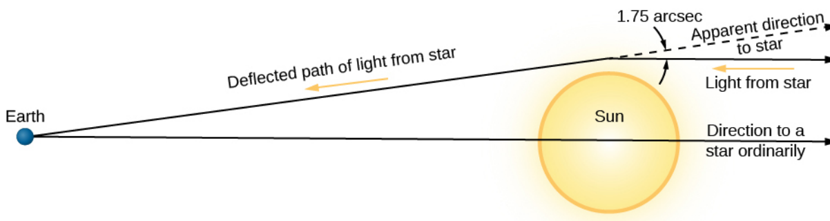
Figure 24.10. Curvature of Light Paths near the Sun. Starlight passing near the Sun is deflected slightly by the “warping” of spacetime. (This deflection of starlight is one small example of a phenomenon called gravitational lensing, which we'll discuss in more detail in The Evolution and Distribution of Galaxies .) Before passing by the Sun, the light from the star was traveling parallel to the bottom edge of the figure. When it passed near the Sun, the path was altered slightly. When we see the light, we assume the light beam has been traveling in a straight path throughout its journey, and so we measure the position of the star to be slightly different from its true position. If we were to observe the star at another time, when the Sun is not in the way, we would measure its true position.
