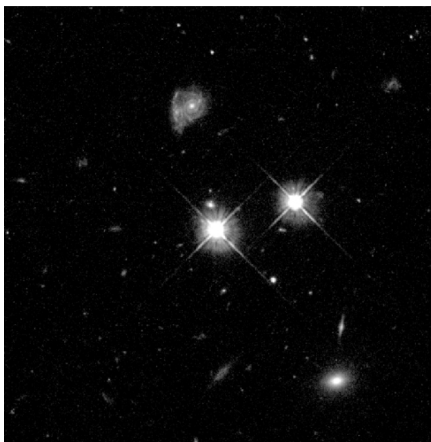
Figure 27.4. Typical Quasar Imaged by the Hubble Space Telescope. One of these two bright “stars” in the middle is in our Galaxy, while the other is a quasar 9 billion light-years away. From this picture alone, there’s no way to say which is which. (The quasar is the one in the center of the picture.) (credit: Charles Steidel (CIT)/NASA/ESA)
