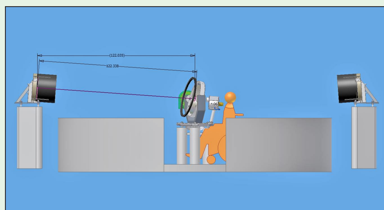
18" primary mirrors set north and south of the larger flat "steering" mirror
