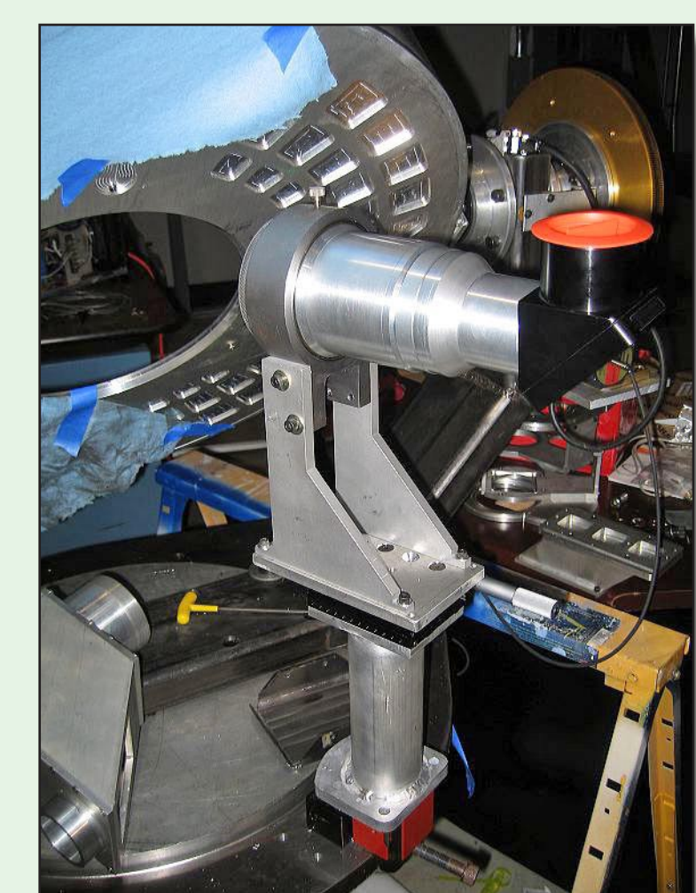
Straight-through monocular with 2" diagonal
