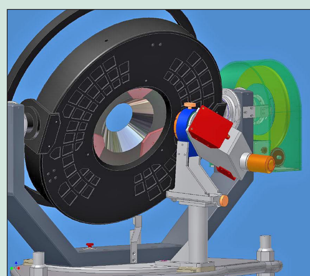
Continuously adjustable periscope viewer rotates about primary optical axis
