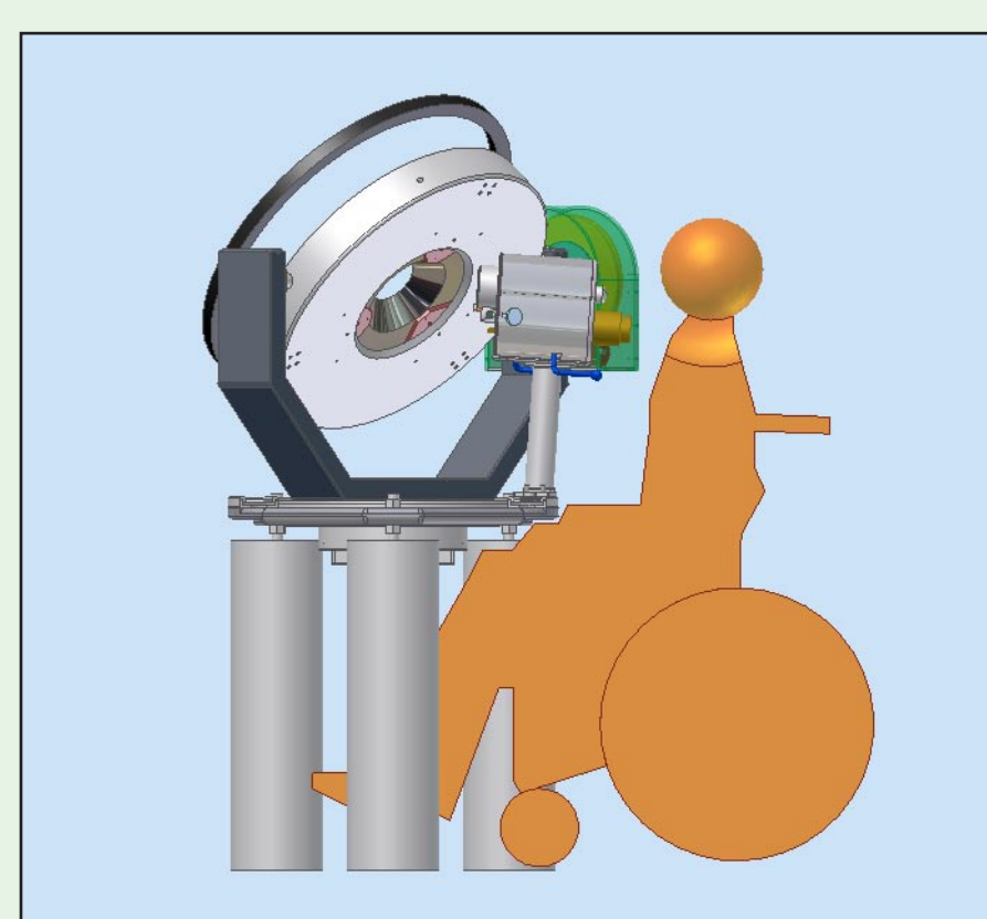
Wheelchair-bound visitors access the telescope simply by rolling up to the eyepiece
