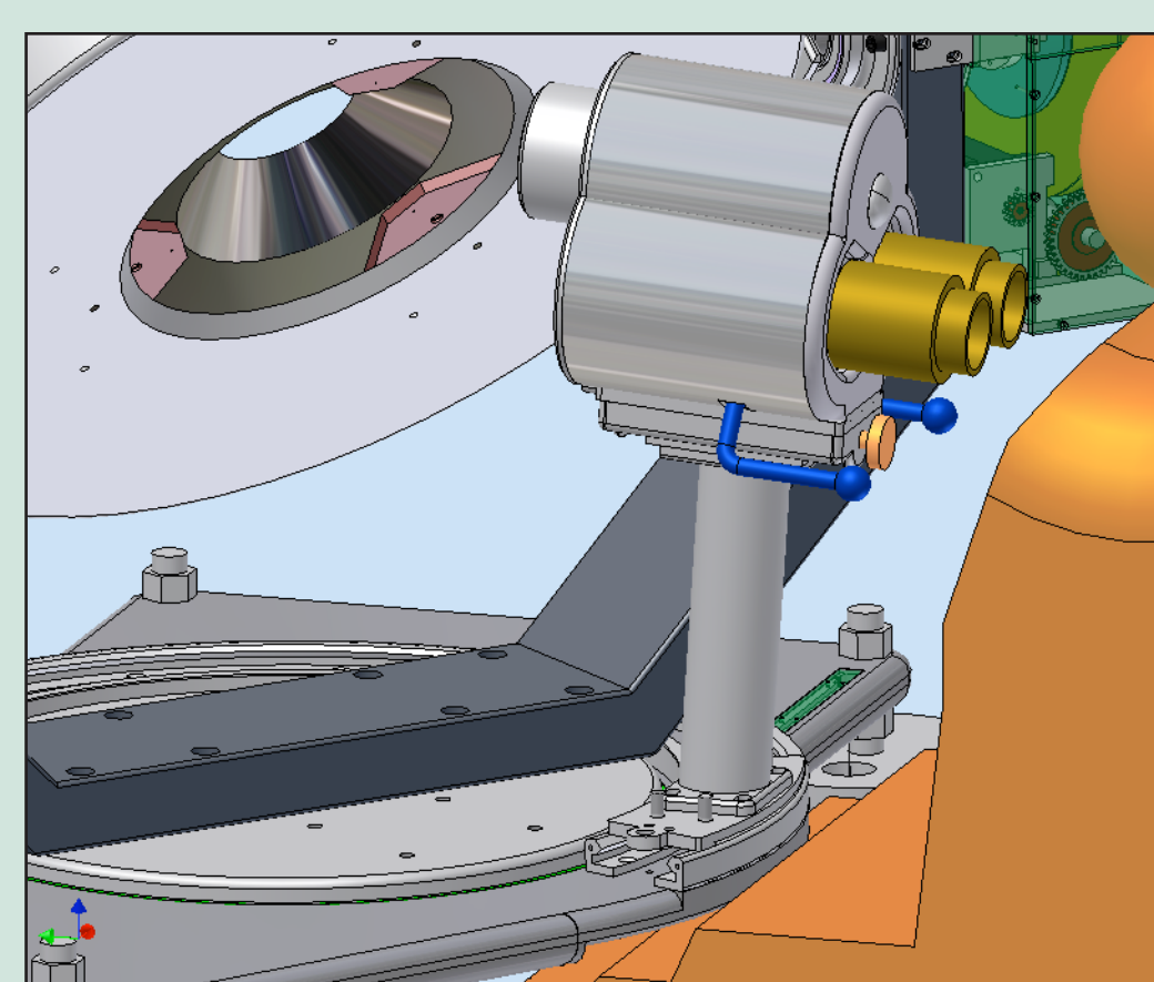
Binocular viewer behind steering flat
