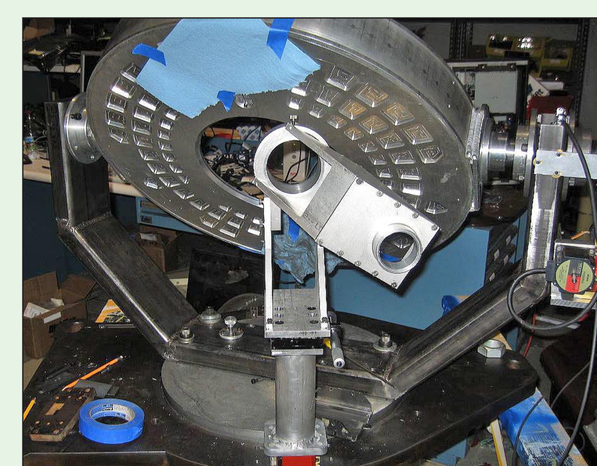
The adjustable periscope viewer awaiting optics
