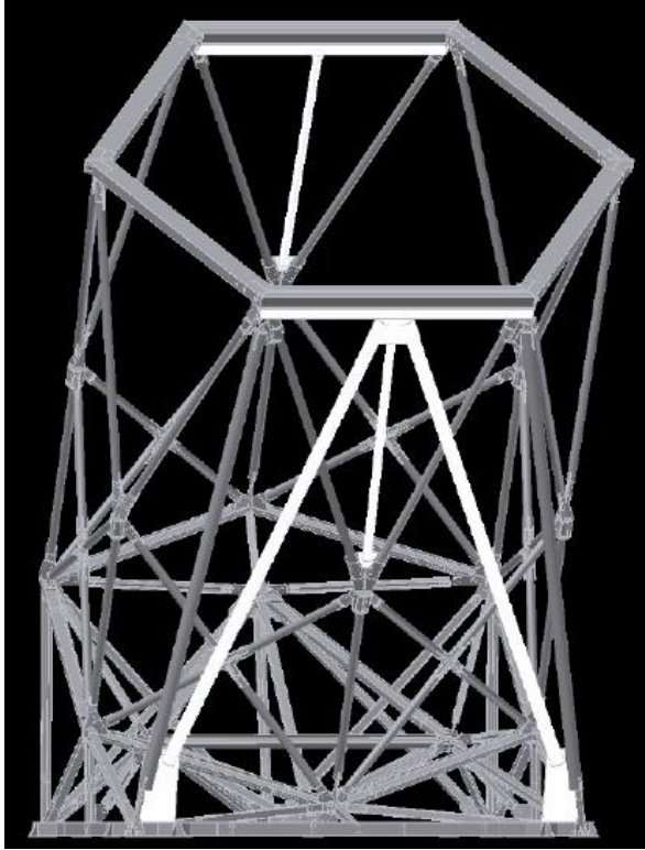
Figure 10: Concept-level modifications to the telescope structure (shown highlighted in white).
