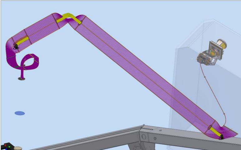
Figure 9: 73 fiber bundles, each carrying 246 fibers must translate through multiple degrees of freedom from the focal surface of the WFC shown at right to each VIRUS unit, one of which is shown to the left within one of the two VIRUS enclosures.
