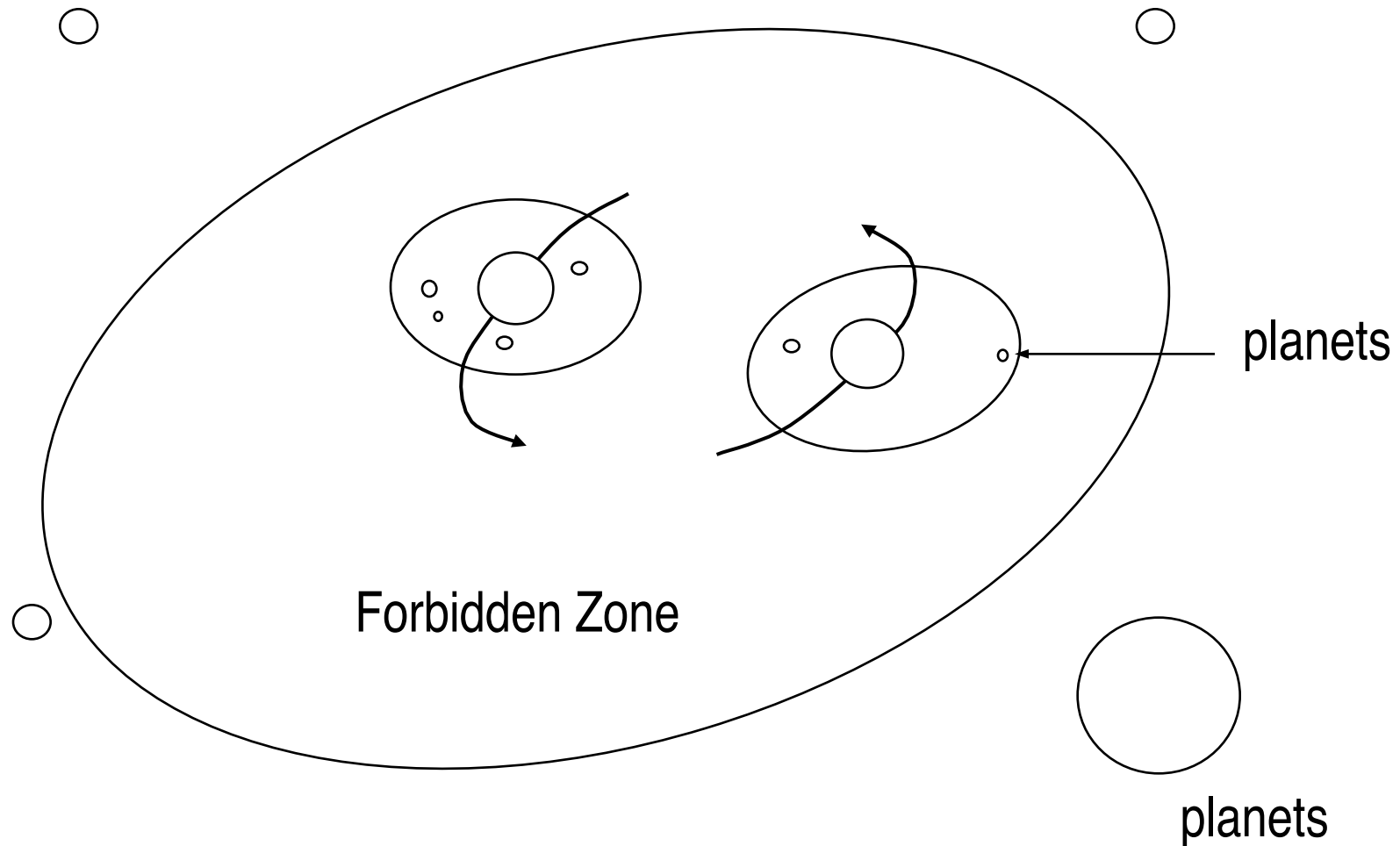
Stable orbits around a Binary Star
