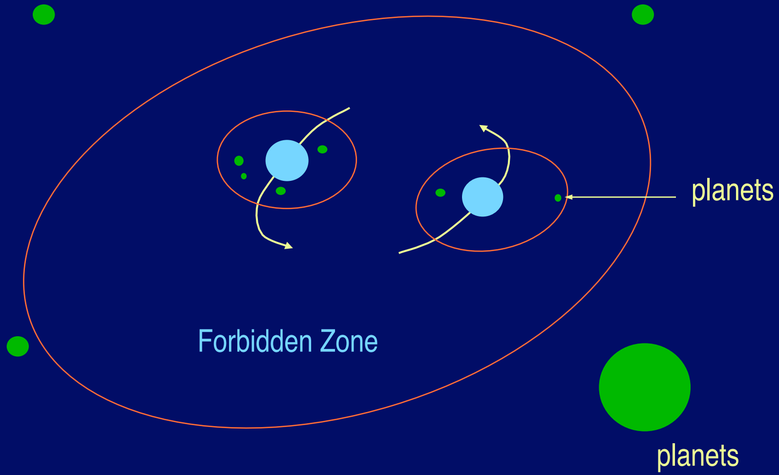
Stable orbits around a Binary Star
