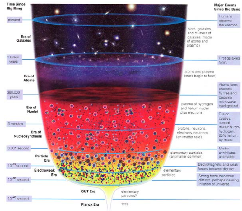
This diagram summarizes the eras of the universe. The names of the eras and their ending times are indicated on the left, and the state of matter during each era and the events marking the end of each era are indicated on the right.
